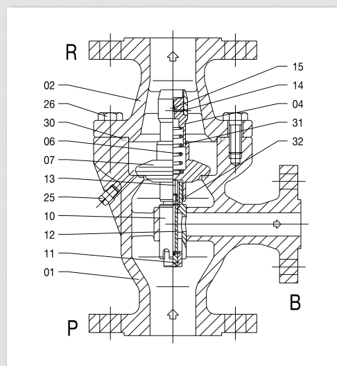
Drain screw pos. 25 as option (standard valve without).
