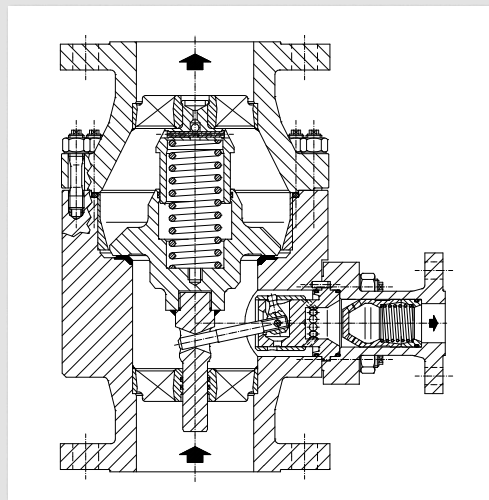
Sectional drawing of an Automatic Recirculation Valve type TDL
