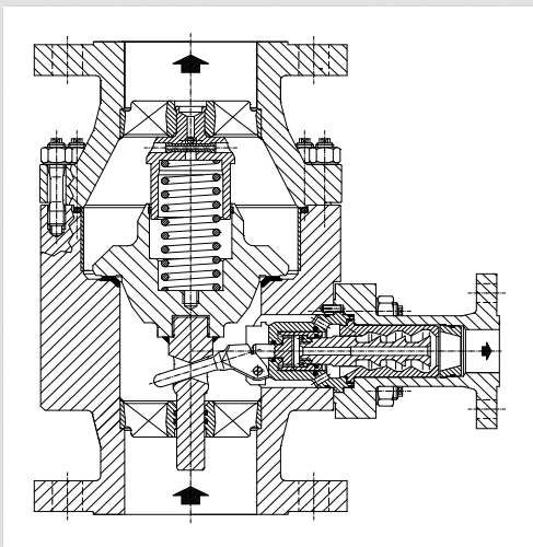
Sectional drawing of an Automatic Recirculation Valve type TDM
